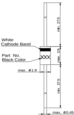
Glass case JEDEC DO-34 Dimensions in mm
